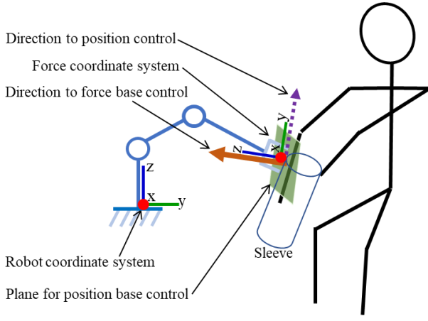
Fig. 4 Switching from position control to hybrid control during putting an arm through the sleeve of clothes
