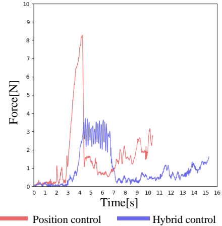
Fig. 9 Applied force comparison between only position-based control and hybrid control
