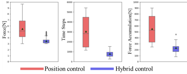
Fig. 6 The boxplot pictures of experimental results. The green triangle is the average value. The rhombus is outlier.
