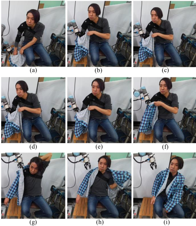
Fig. 7 Examples of putting an arm through the sleeve of shirt by an autonomous robot at the time of contact
