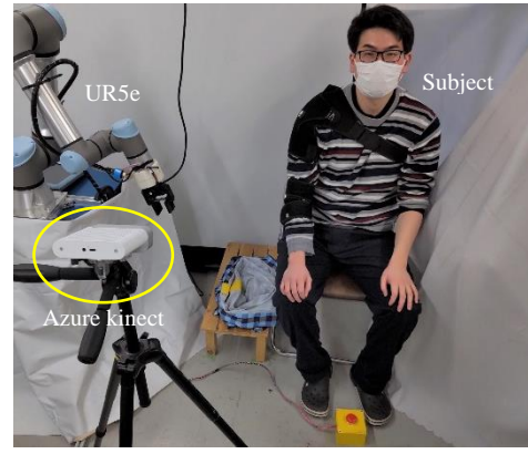
Fig. 5 Arrangement of robot and sensors in the experiment.
