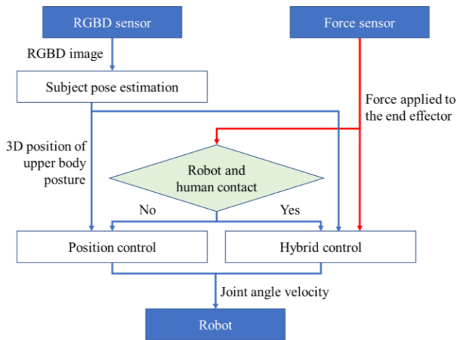
Fig. 2 Functional configuration of the proposed system
